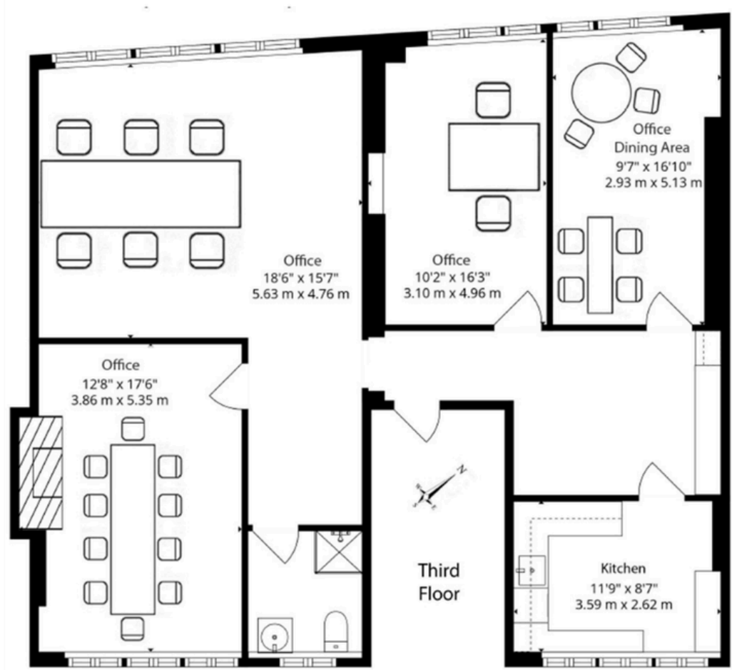
3rd Floor – 1,322 sq ft
